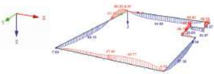
Figure 13. Diagram of the moments M_{Ed} acting on the strip foundations expressed in kNm.
