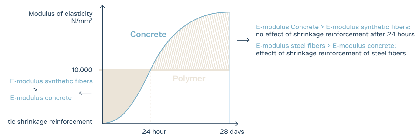
Figure 16. The evolution of the concrete modulus of elasticity during the first 28 days after pouring.
