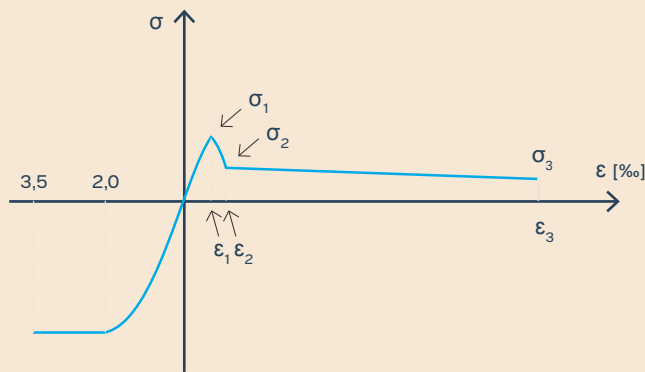
Figure 7. Stress-strain (σ-ε) relationship used for design of SFRC.
