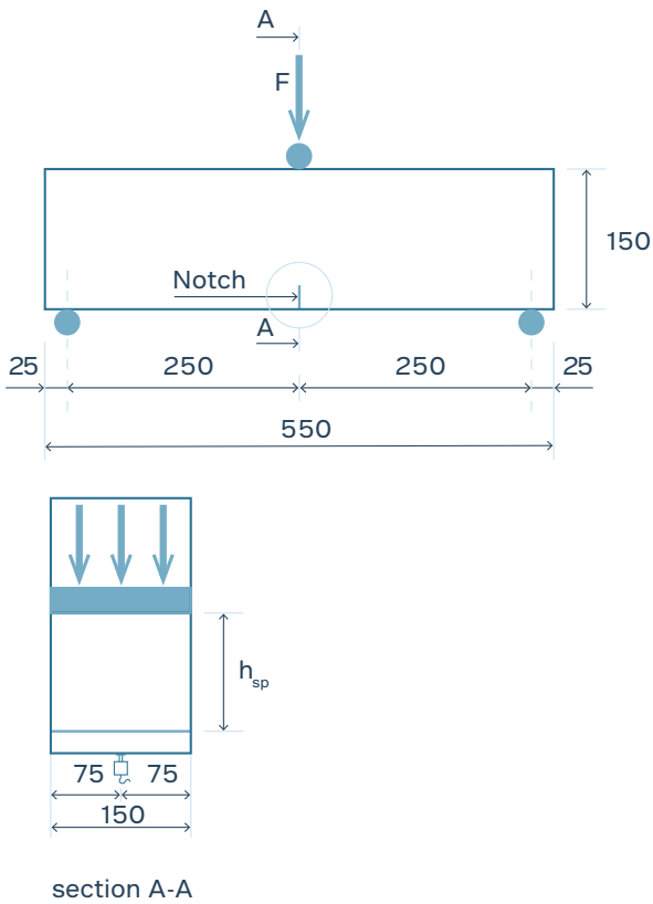
Figure 4: Setup of the three-point bending test according to EN 14651 [5], dimensions in mm.
