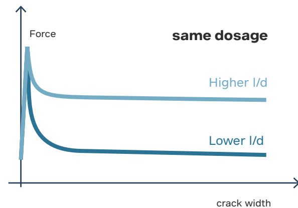
Figure 3. Effect of l/d-ratio on the flexural performance.
