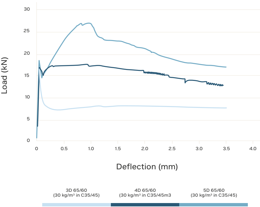
Figure 6. Effect of the Damix® series on the load-deflection response of an EN14651 beam test.
